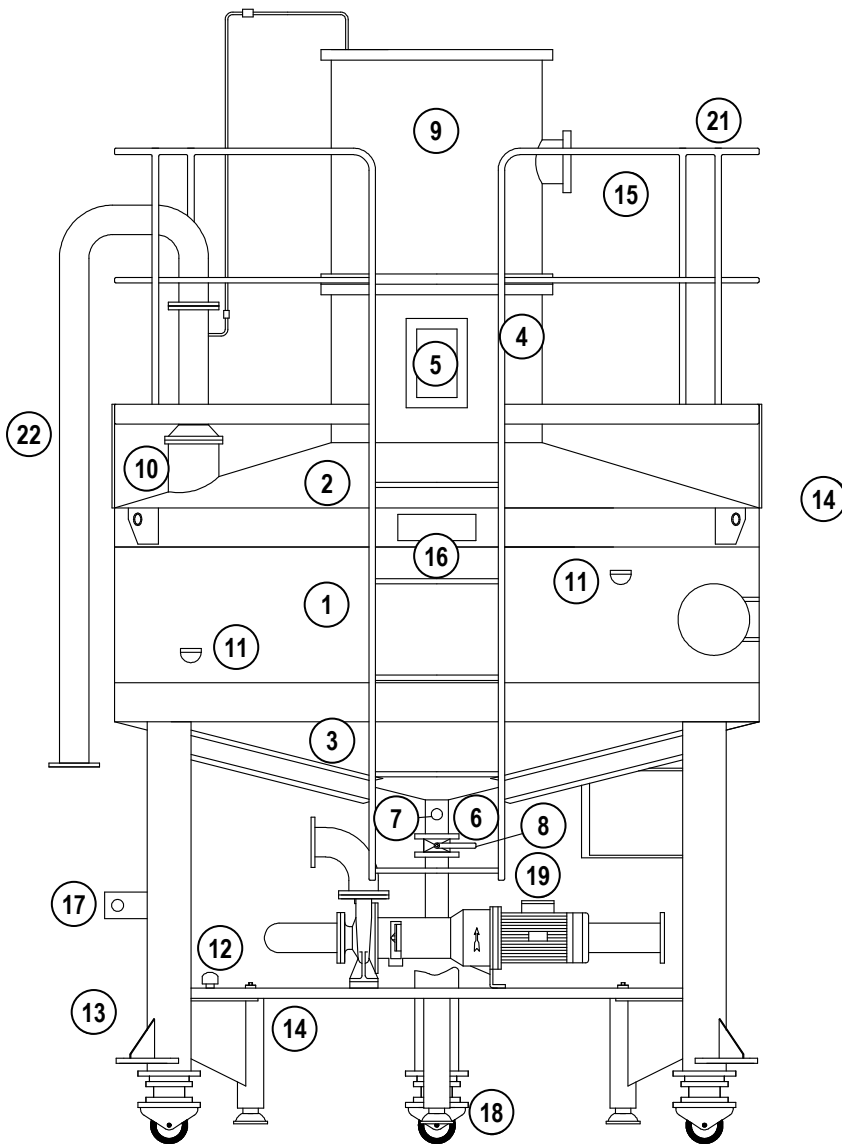
TYPICAL DRAWING OF A 5.000 LITRES TANK PROVER WITH DIFFERENT OPTIONS
